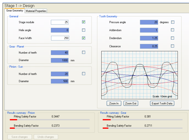
Figure 4 The initial design dialog for determine the geometry of the stage
