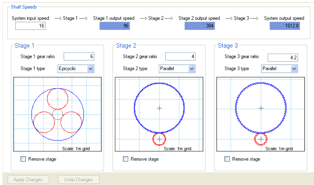
Figure 3 The system overview with 3 gear stages
