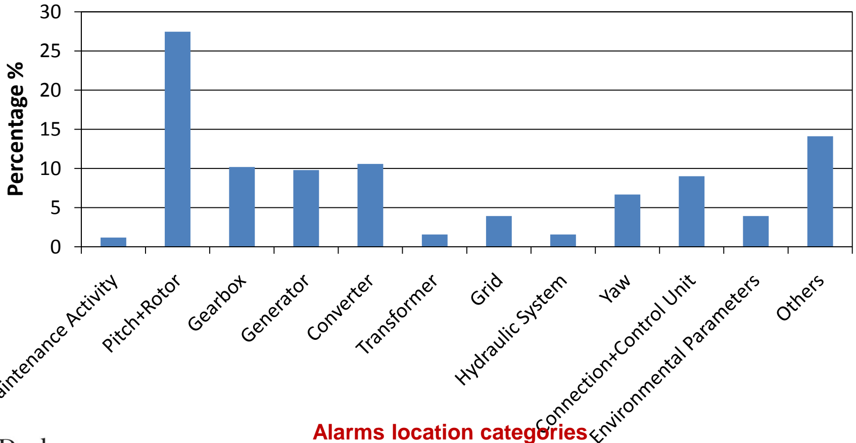
The Ratio of Alarms in Each Category to the Total Numbers of Alarms of a WT
