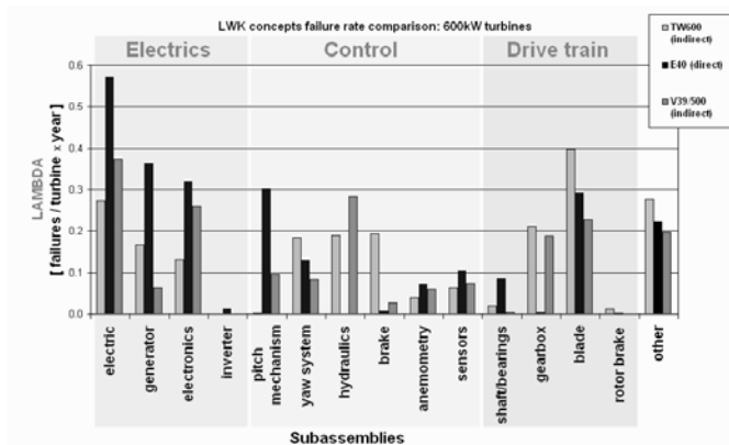
Figure 3: Comparison between failure rates of the Group 1, smaller WT Concepts
