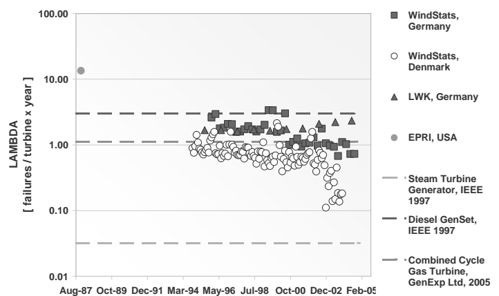
Figure 1: The failure rates of Onshore Wind Turbines taken from WindStats [4] and compared with other power sources.
