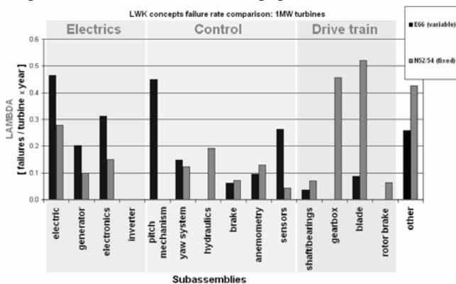
Figure 4 : Comparison between failure rates of the Group 2, larger, WT Concepts
