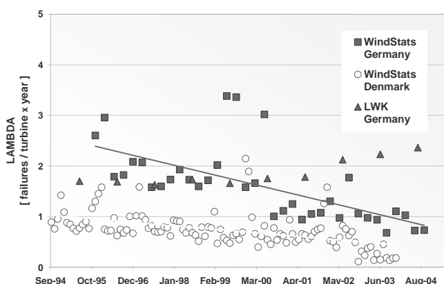
Figure 2: The failure rates of Onshore Wind Turbines taken from LWK [9] and compared with rate of onshore Wind Turbines taken from WS [4].
